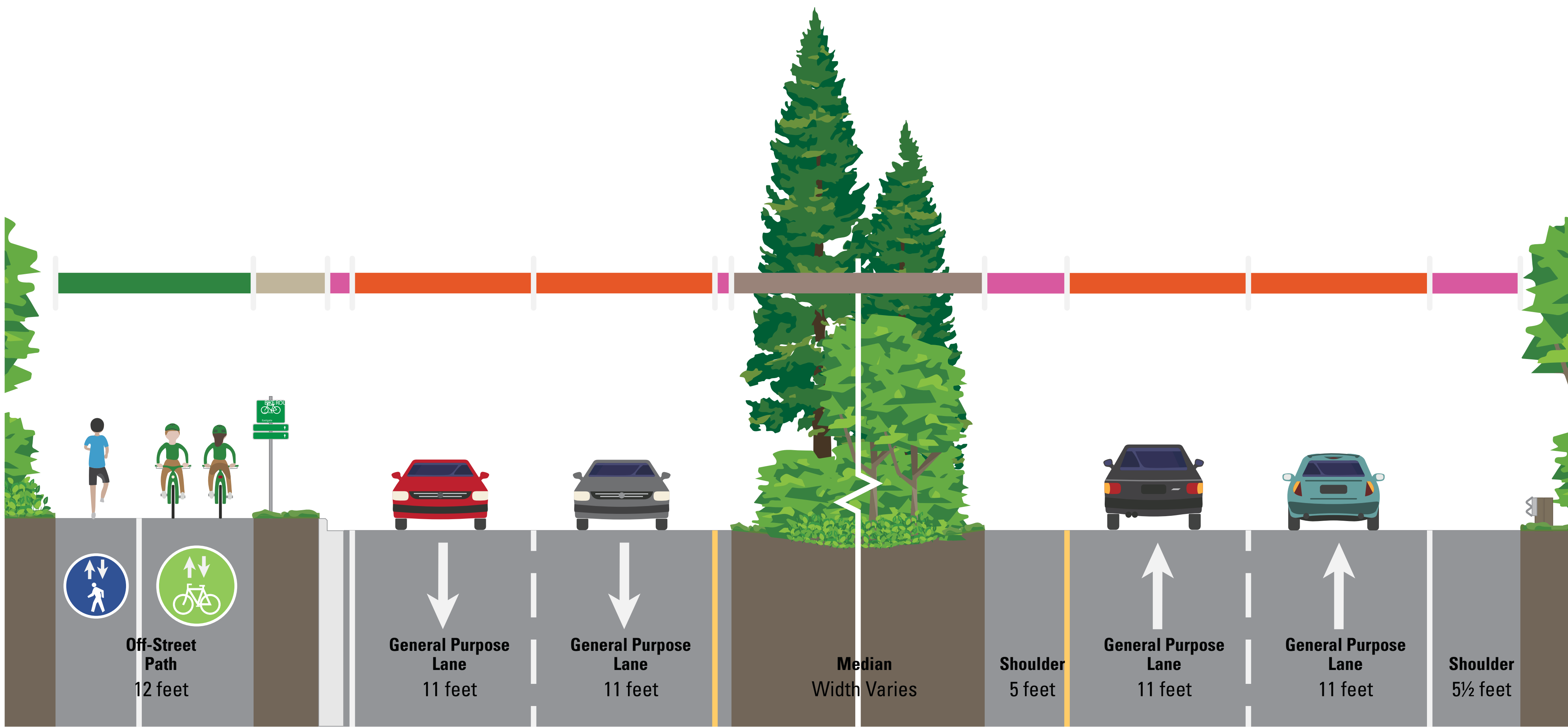
OFF-STREET PATH CONCEPT
