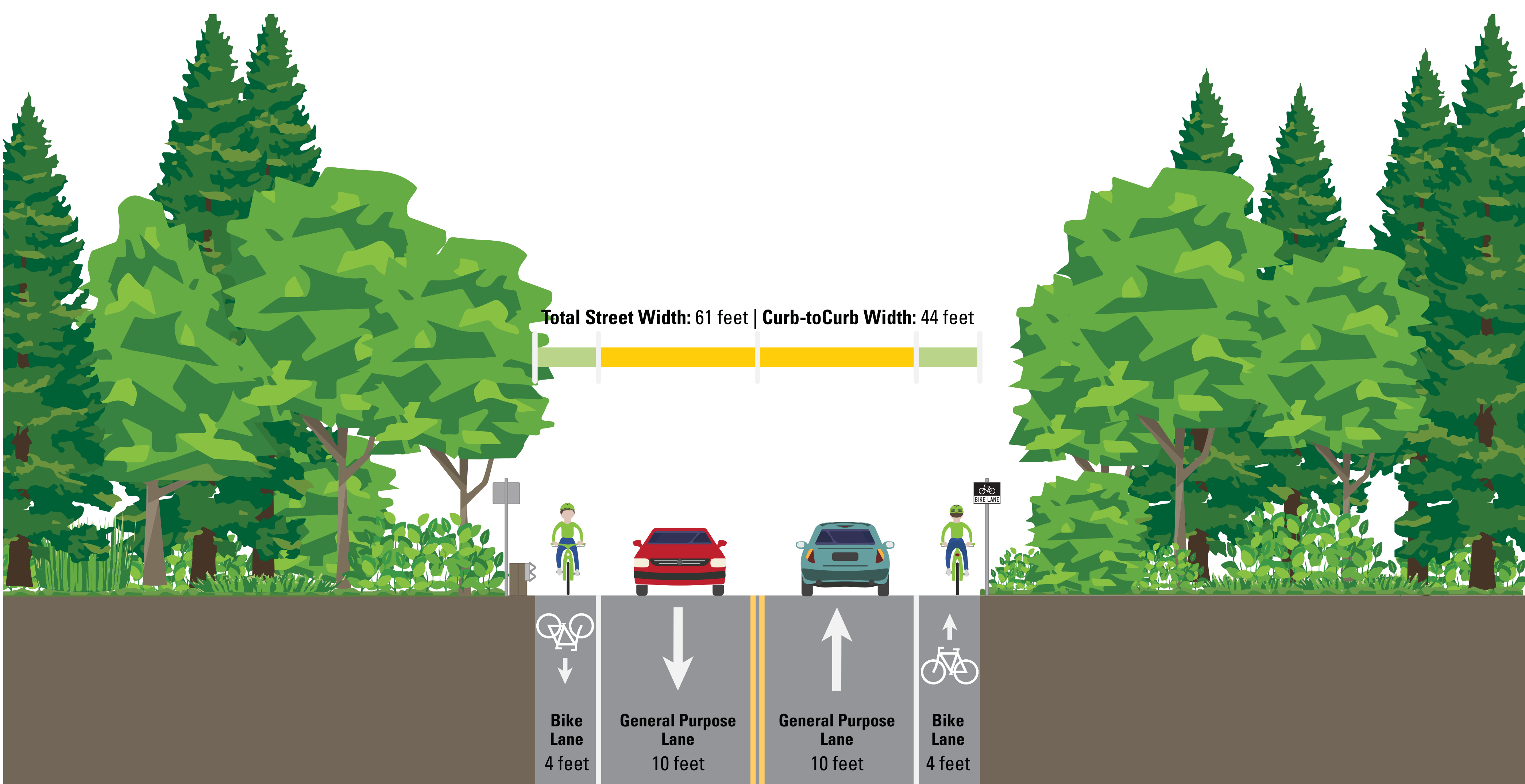
CONVENTIONAL BIKE LANE CONCEPT
