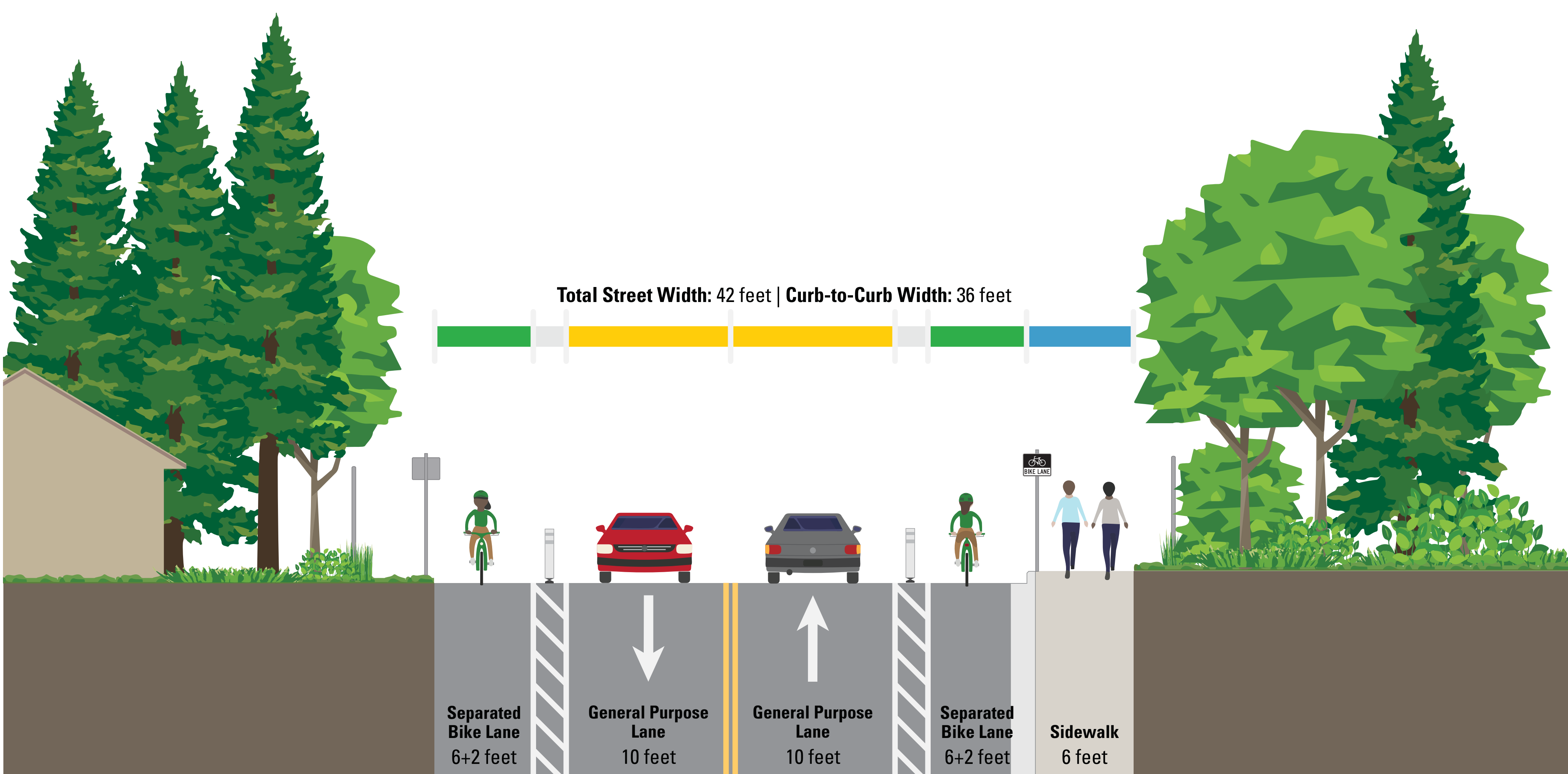
SEPARATED BIKE LANE CONCEPT
