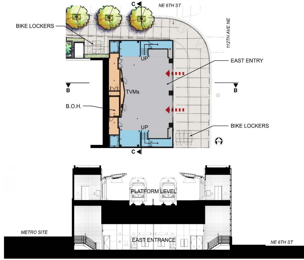
SECTION C-C
