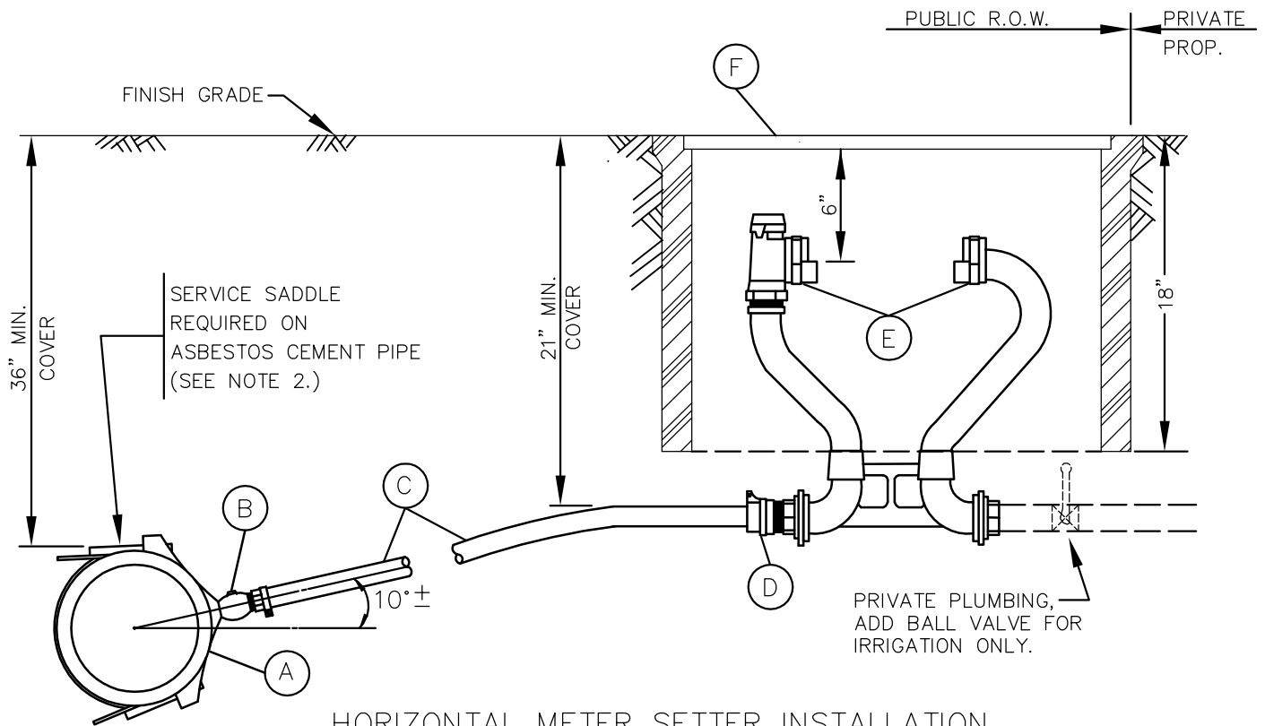
HORIZONTAL METER SETTER INSTALLATION
