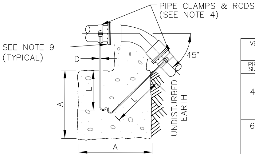
VERTICAL BLOCKING FOR 45° BENDS
