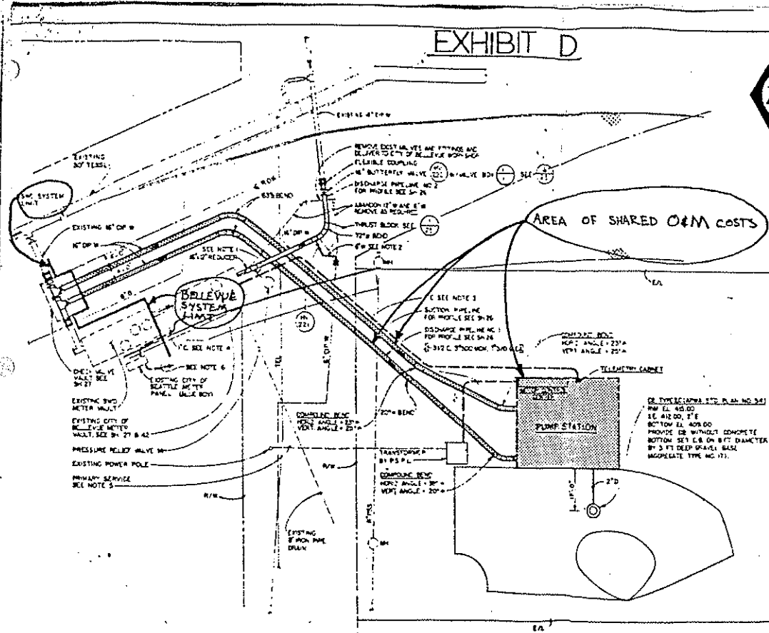
YARD PIPING AND ELECTRICAL CONDUIT PLAN SCALE 1\"/>
