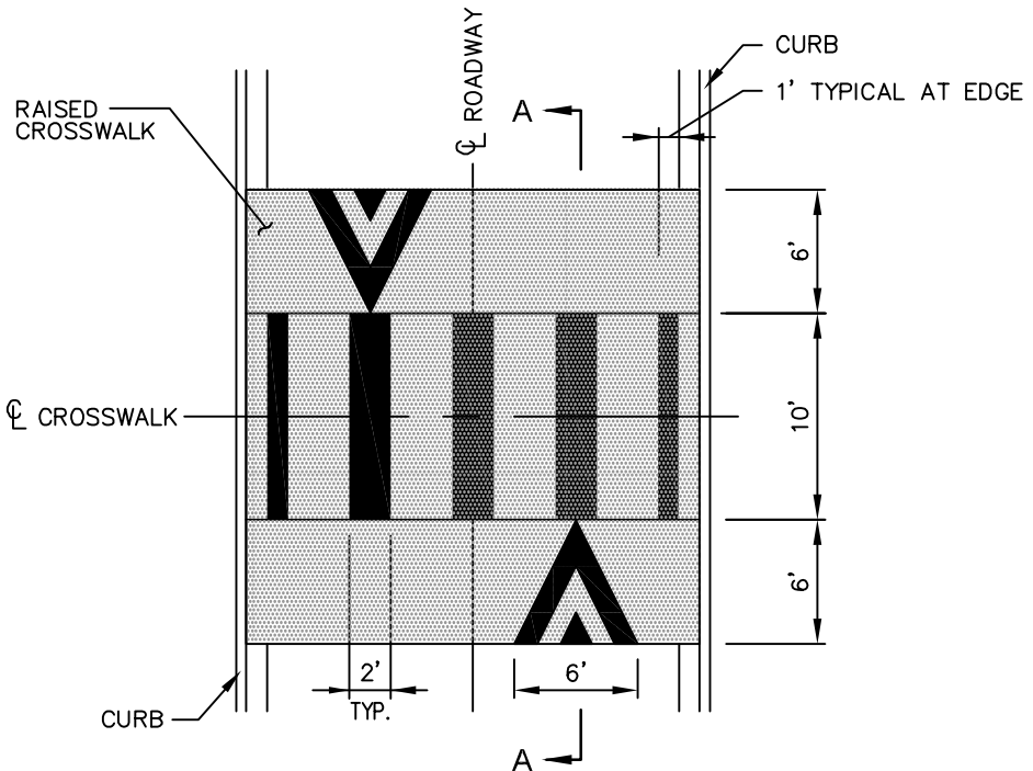
MARKING DETAIL
