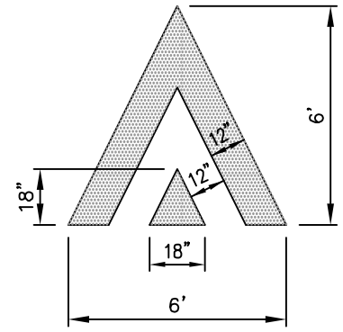
CHEVRON DETAIL
