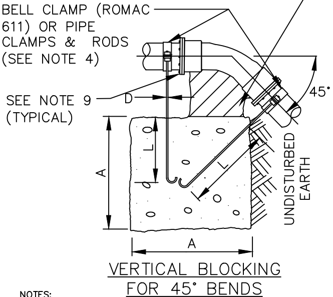
VERTICAL BLOCKING SIZE W/RESTRAINED JOINTS SOIL TYPE = COHESIVE GRANULAR [GC+SC] SAND, GRAVEL, CLAY MIXTURE
