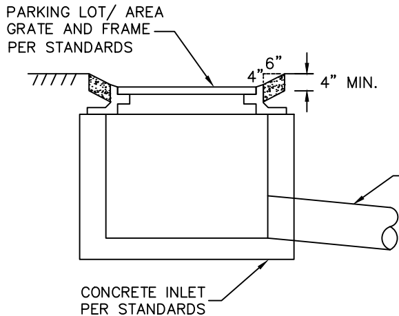
PRESSURE RELIEF DRAIN
