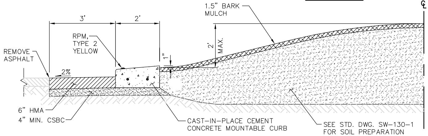
TYPICAL SECTION
