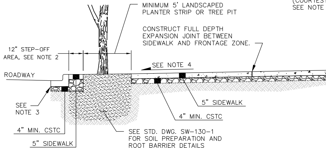
SECTION B-B
