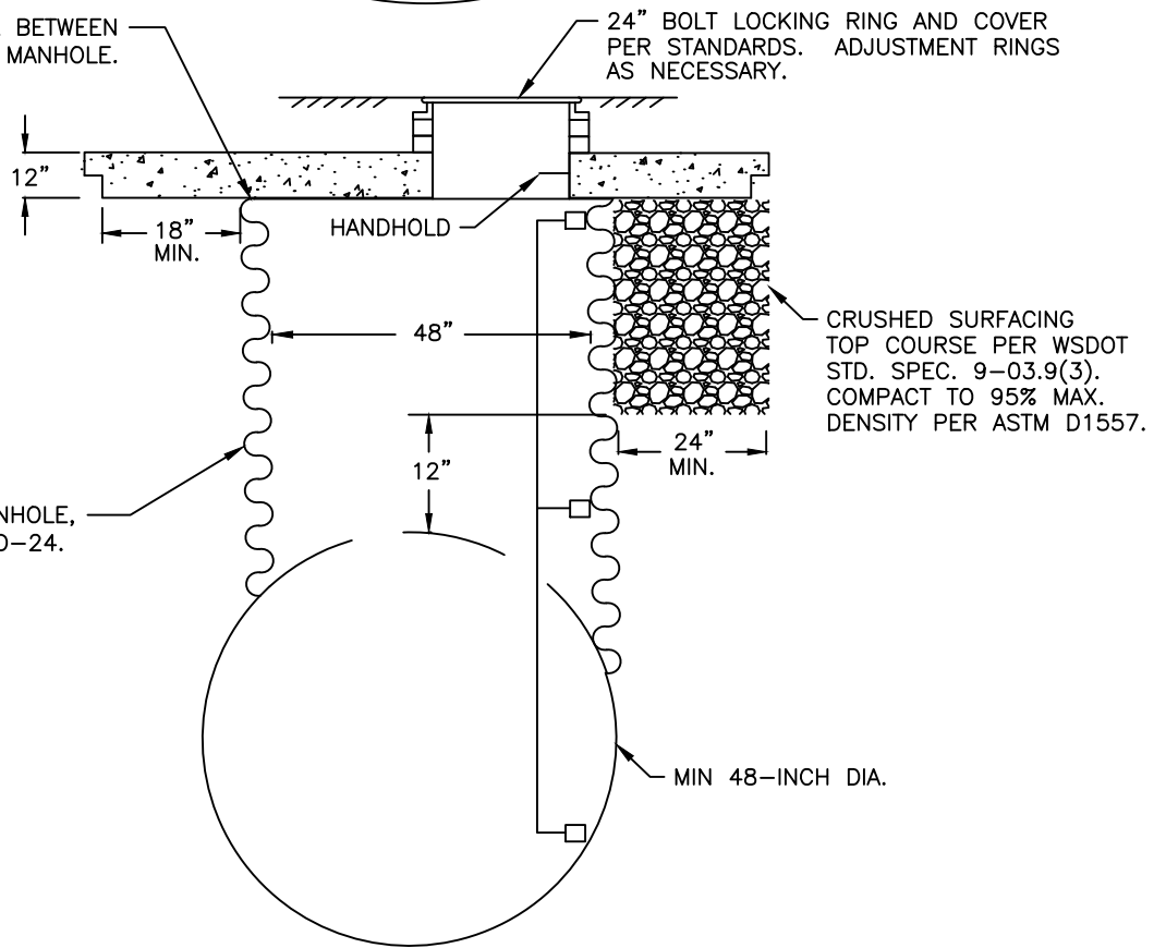
ECCENTRIC SECTION
