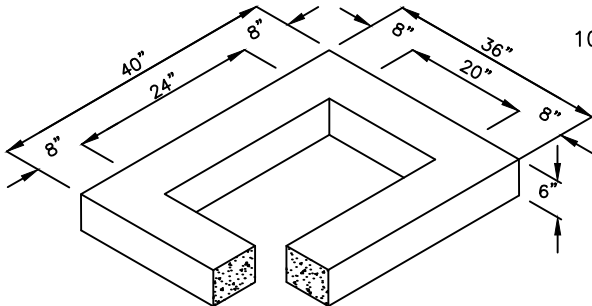
6" REDUCING SECTION
