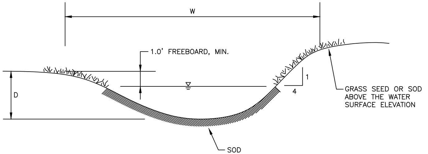
TYPICAL SECTION
