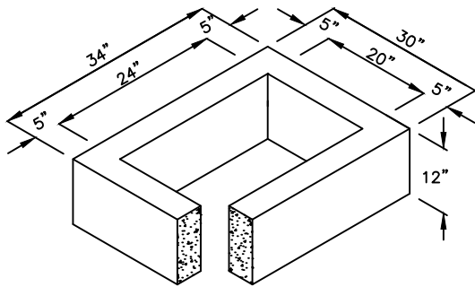
12" RISER SECTION
