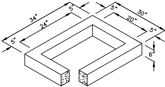
6" RISER SECTION
