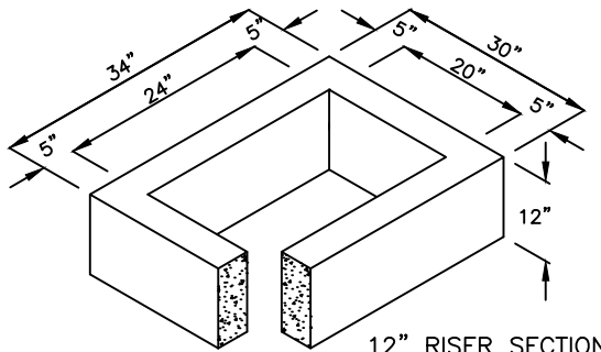
12" RISER SECTION
