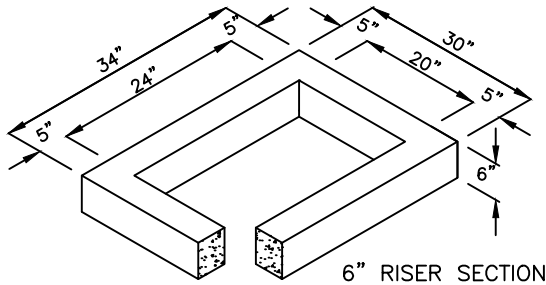
6" RISER SECTION
