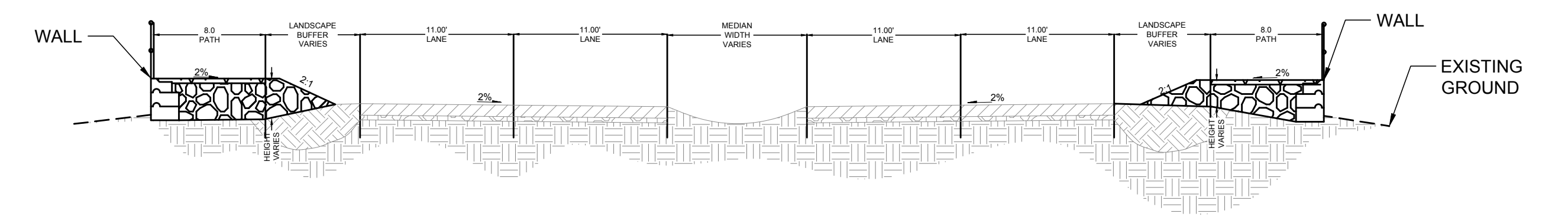
TYPICAL SECTION NTS
