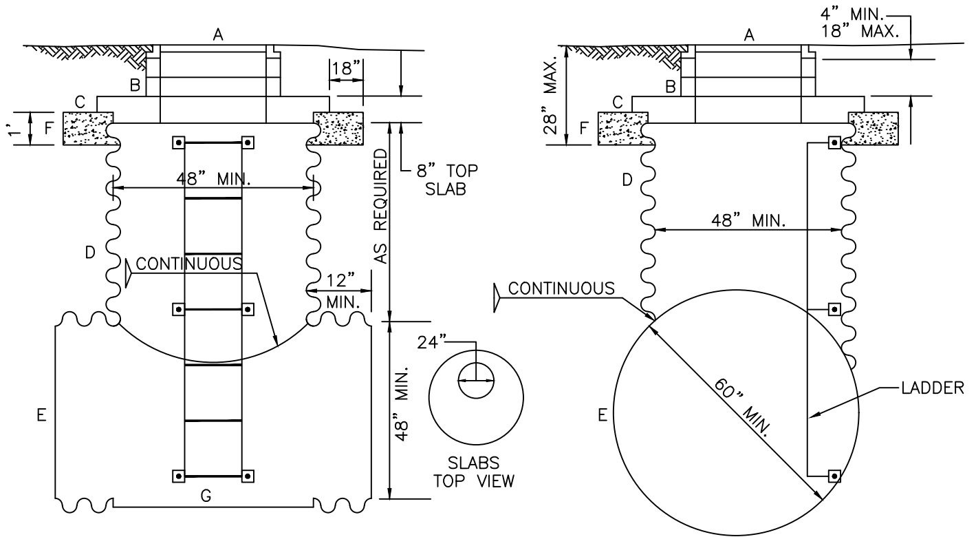
CONCENTRIC ELEVATION
