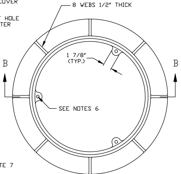
RING PLAN
