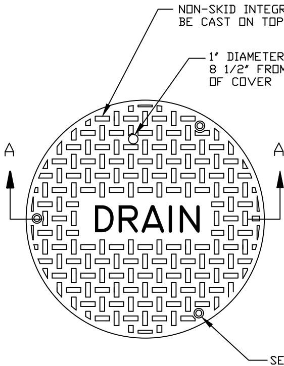
COVER PLAN
