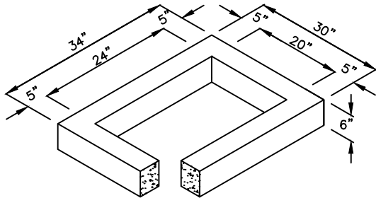
6" RISER SECTION
