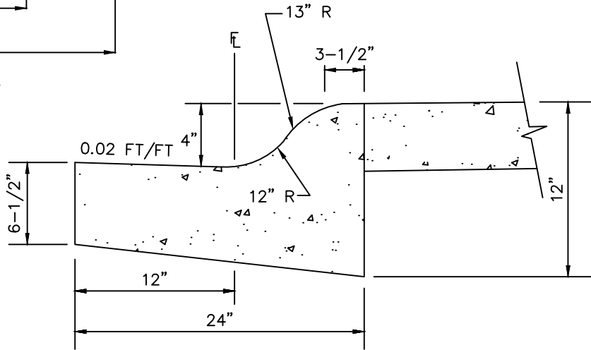
ROLLED CURB
