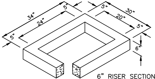
6" RISER SECTION
