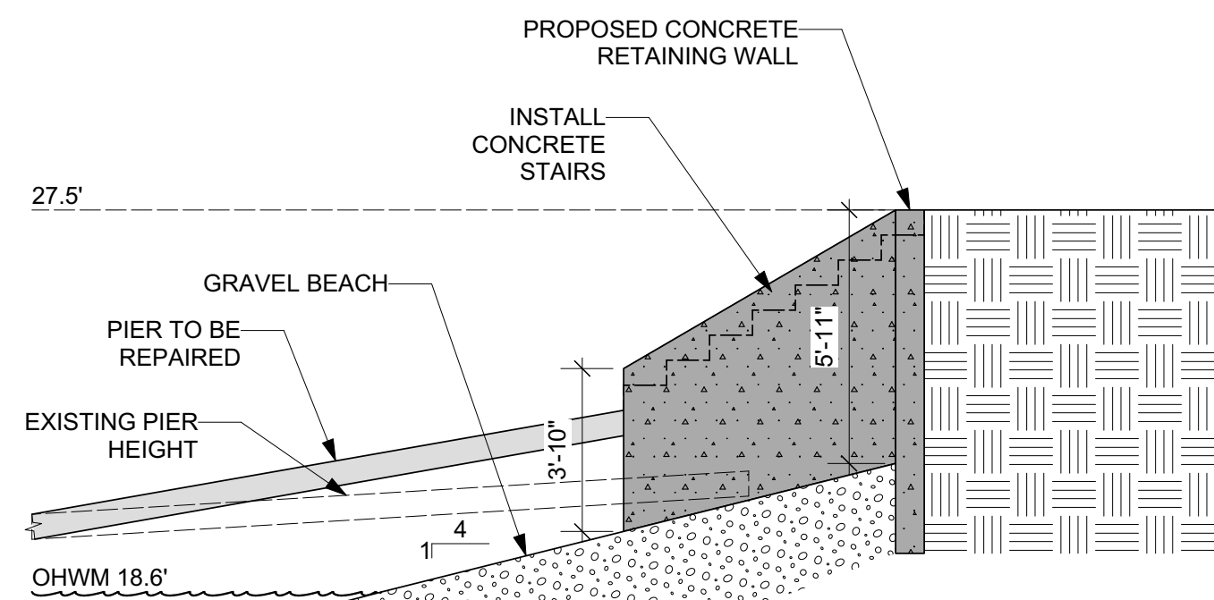
BEACH & RETAINING WALL ELEVATION SCALE 1/4" = 1'-0"
