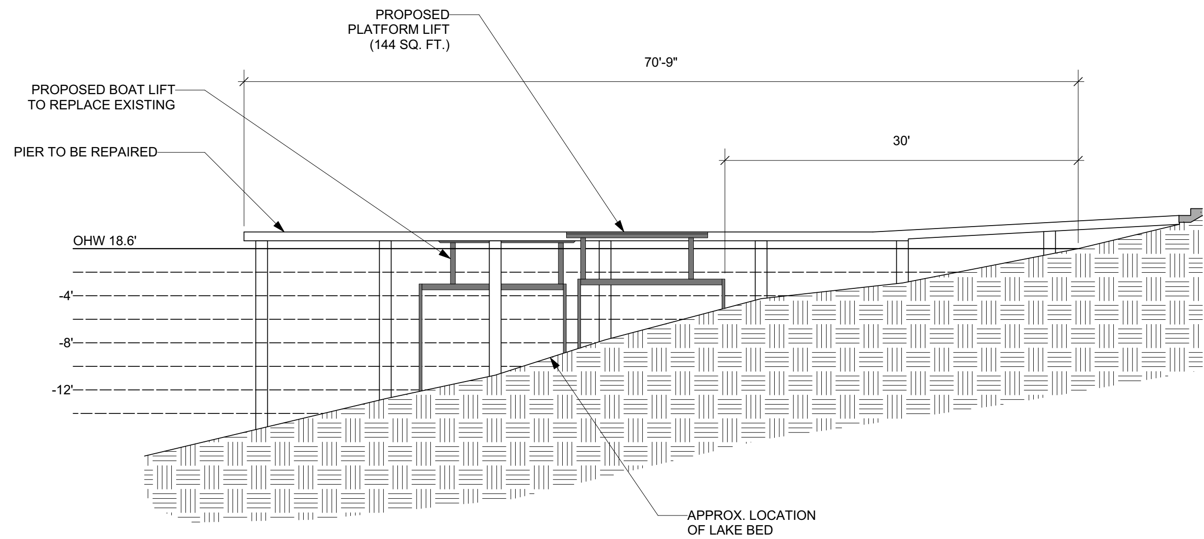
PIER ELEVATION SCALE 1/8" = 1'-0"
