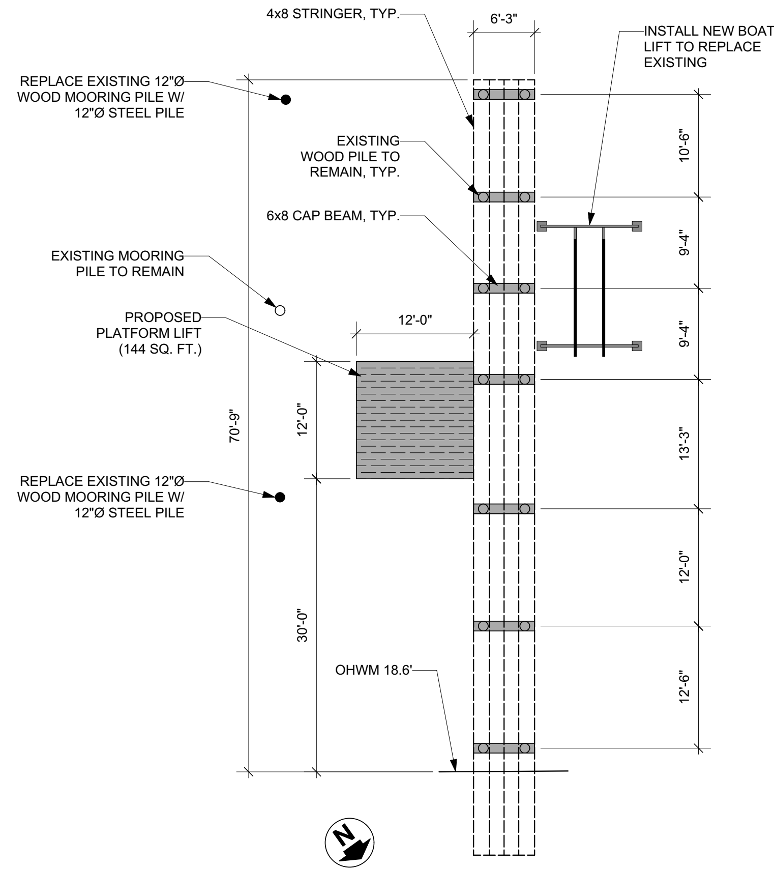
PIER PLAN SCALE 1" = 10'-0"
