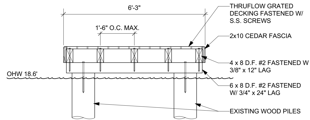
PIER WALKWAY SECTION SCALE 1/2" = 1'-0"
