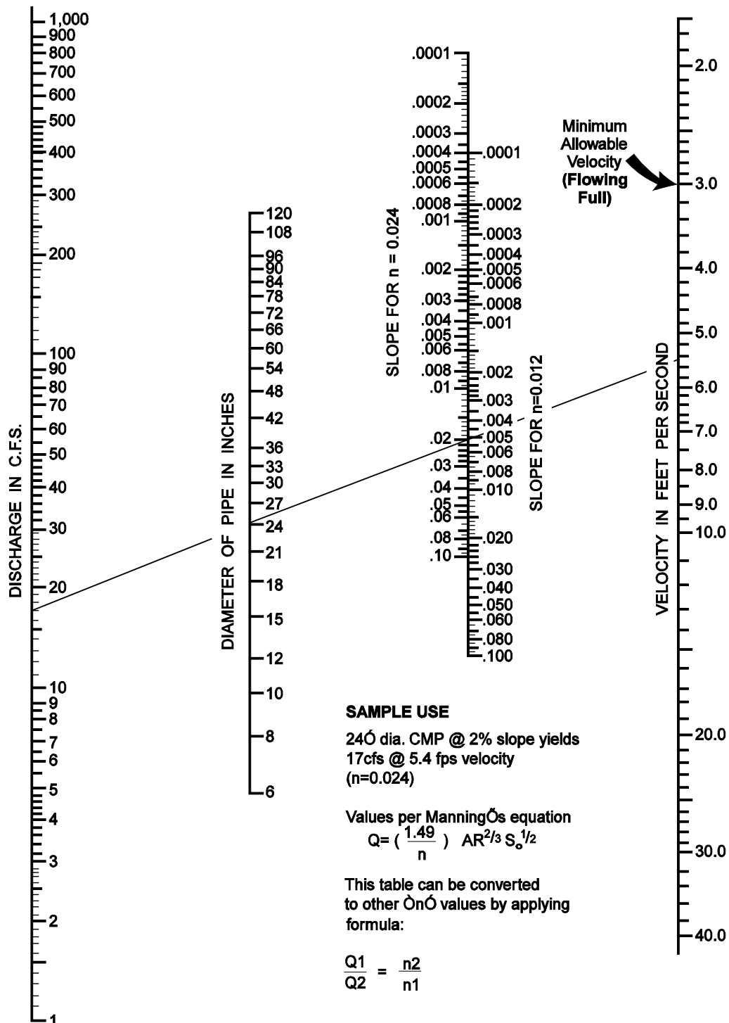
Figure 4.16 Nomograph For Sizing Circular Drains Flowing Full
