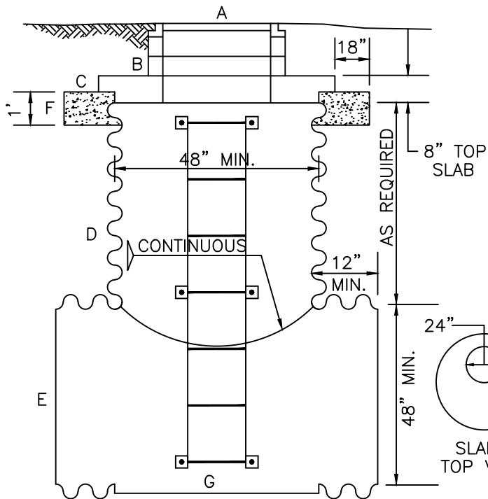
CONCENTRIC ELEVATION
