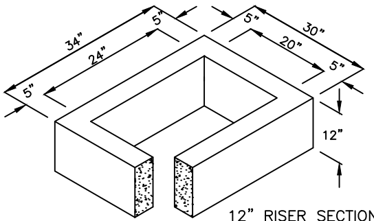
12" RISER SECTION
