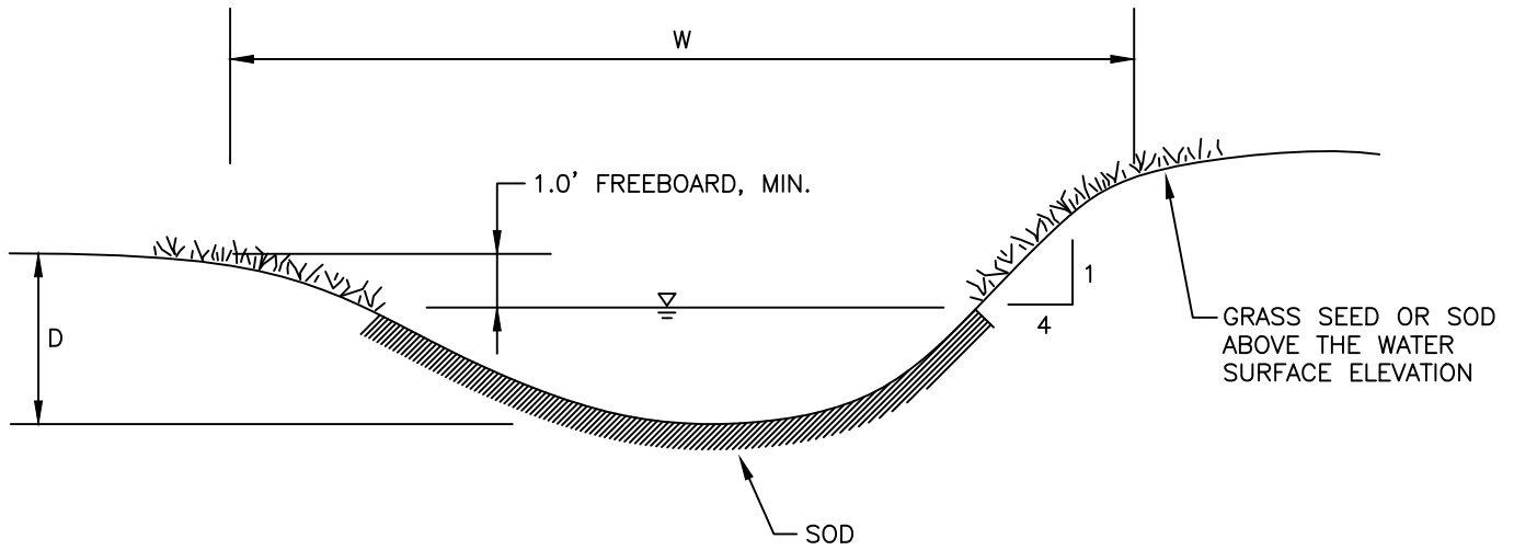
TYPICAL SECTION
