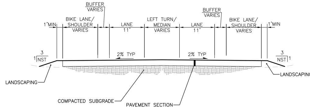
SECTION B - LAKEMONT BLVD SE (NON-INTERSECTION AREA) NOT TO SCALE
