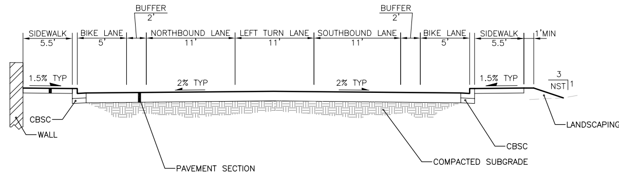
SECTION A - LAKEMONT BLVD SE (INTERSECTION AREA) NOT TO SCALE
