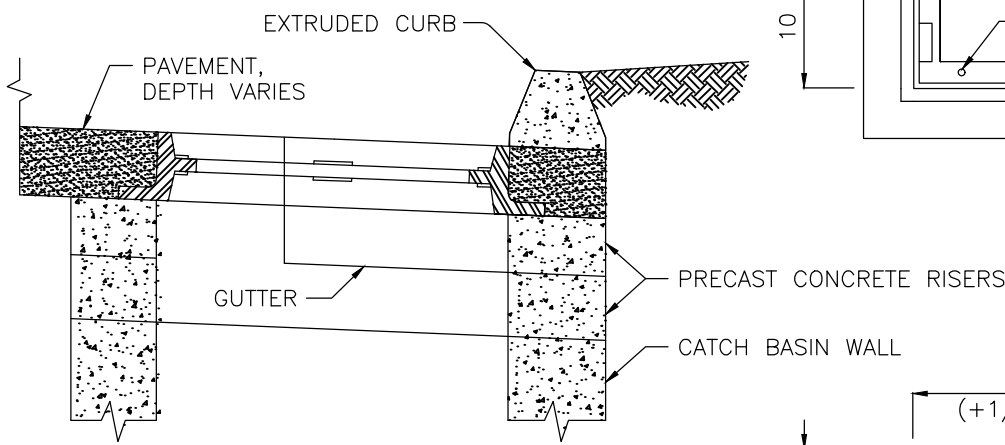
EXTRUDED CURB
