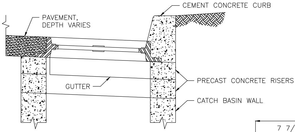
VERTICAL CURB
