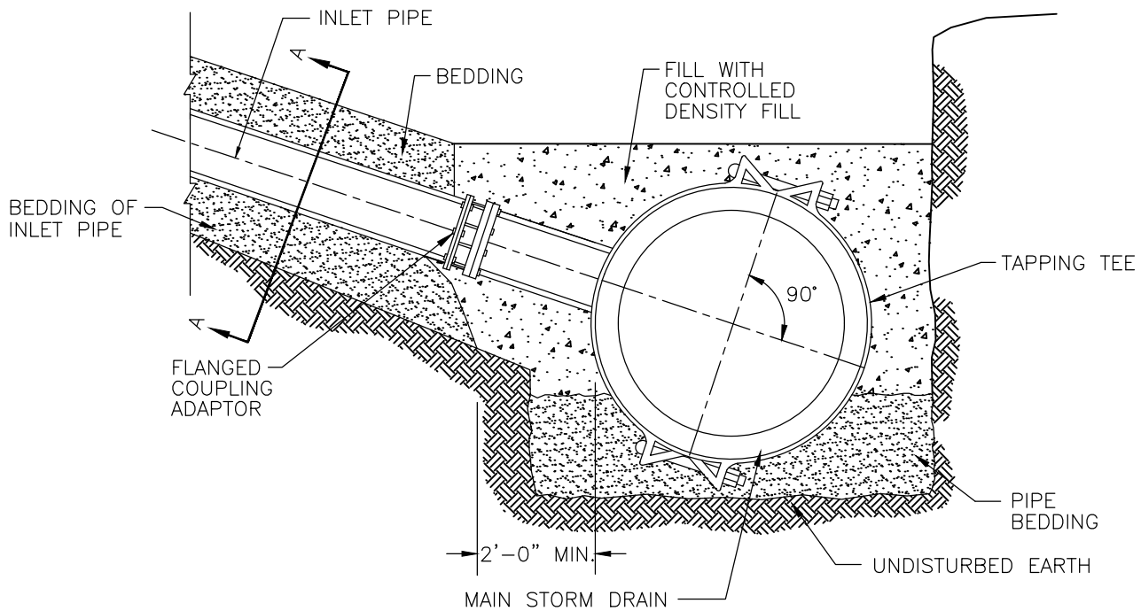
ELEVATION VIEW
