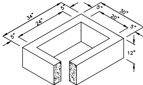
12" RISER SECTION
