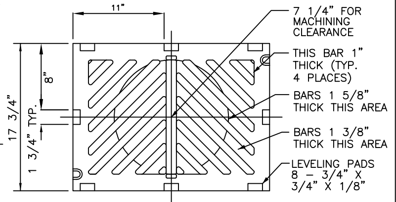
BOTTOM VIEW
