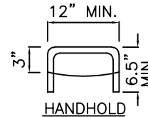
TYPICAL ORIENTATION FOR ACCESS AND STEPS
