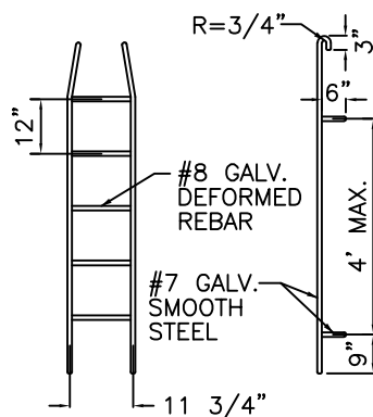
PREFABRICATED LADDER
