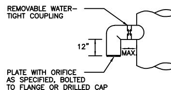
ELBOW DETAIL
