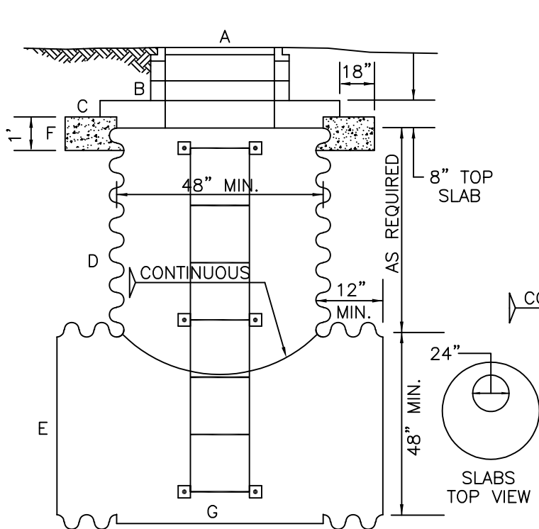
CONCENTRIC ELEVATION
