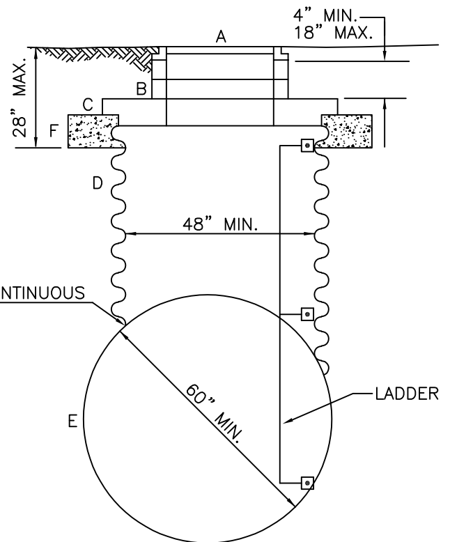
ECCENTRIC SECTION
