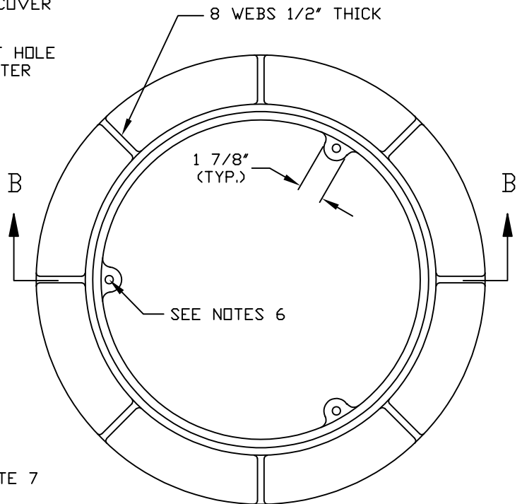
RING PLAN
