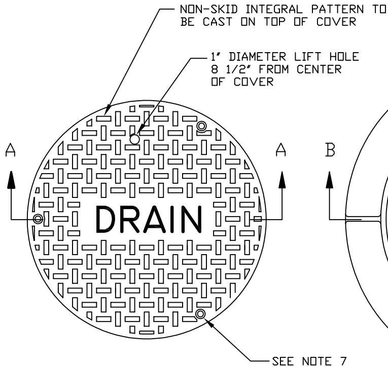
COVER PLAN
