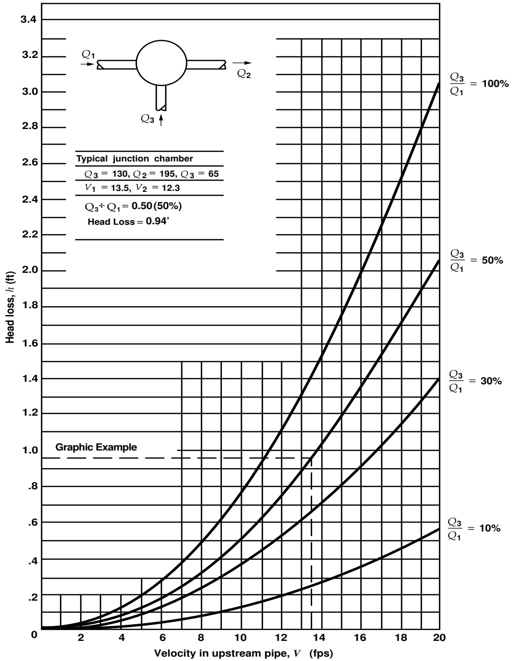
Figure 4.21 Junction Head Loss In Structures
