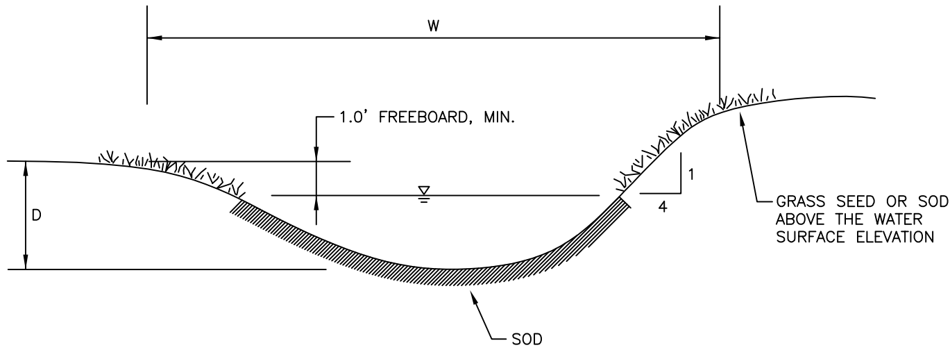
TYPICAL SECTION
