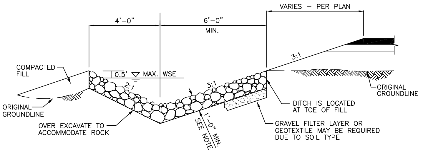
ROCK-LINED SHOULDER DITCH IN FILL SECTION
