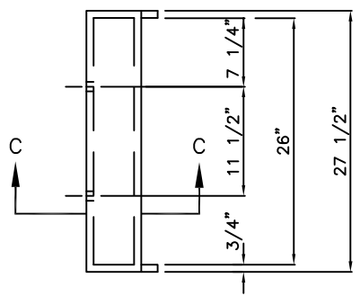
HOOD DETAIL
