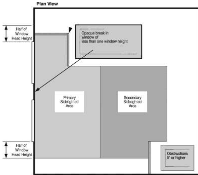
Computing the secondary sidelighted area.
