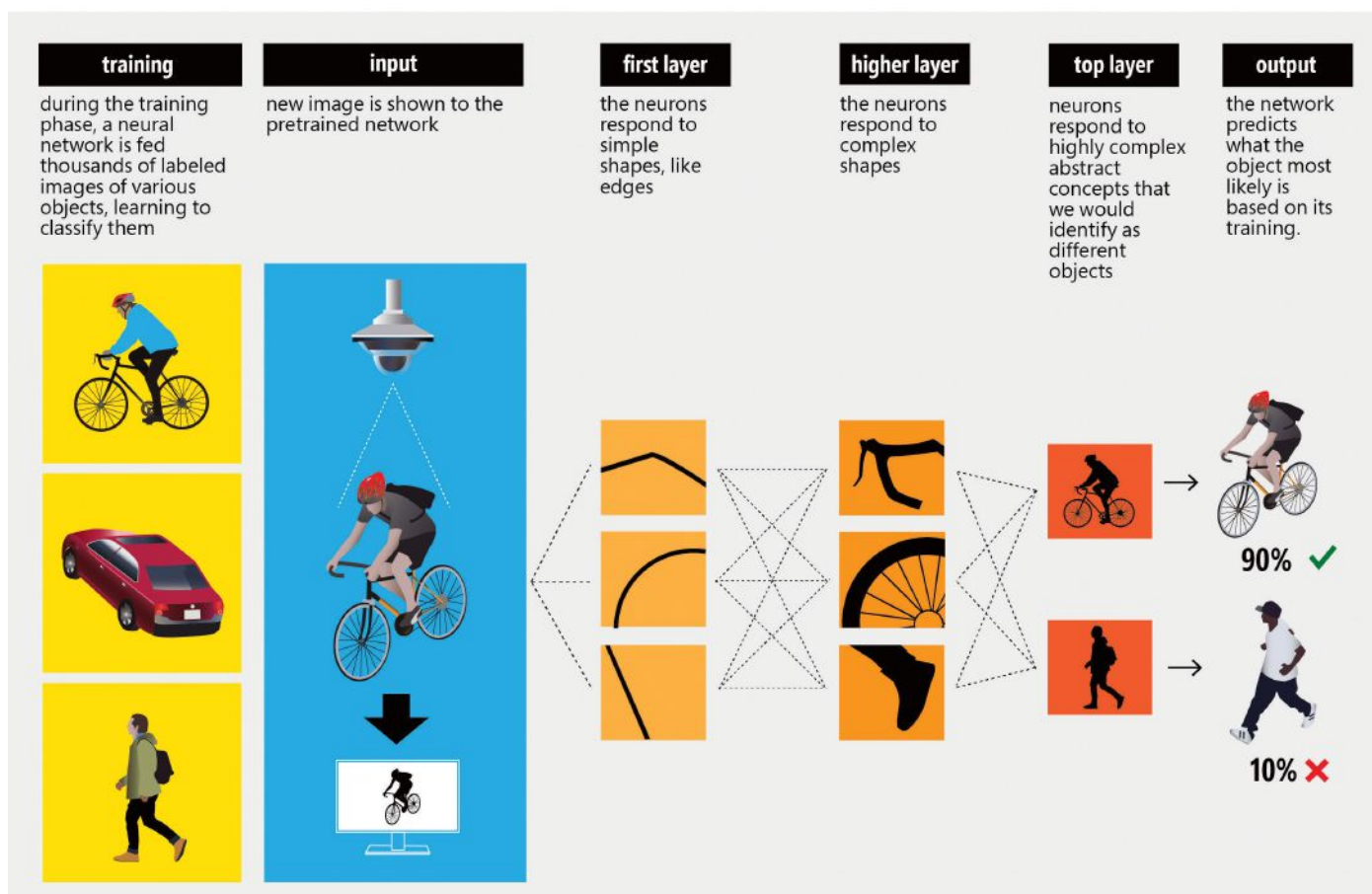
Figure 5. Graphic showing how objects are classified using a Deep Neural Network.
