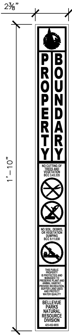
DECAL (3" = 1'-0")
